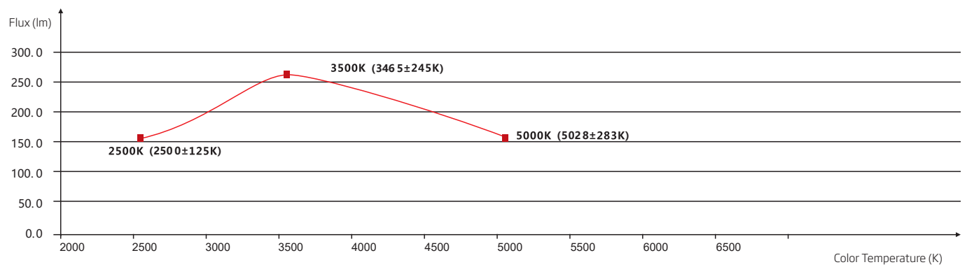
Luminous Flux vs. CCT
